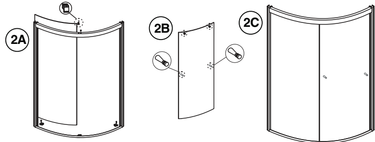
SLIDING GLASS PANEL INSTALLED ON RIGHT
