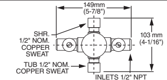
THREADED (STOPS) (R115SS)
