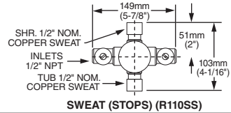
SWEAT (STOPS) (R110SS)
