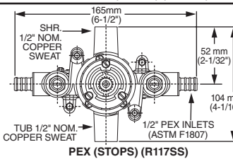
PEX (STOPS) (R117SS)
