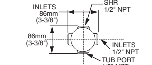
THREADED (R125)
