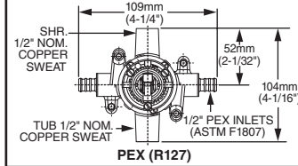
PEX (R127)
