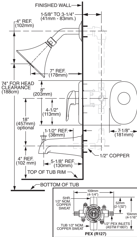
PEX (R127)
