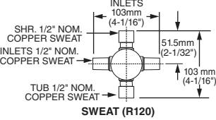
SWEAT (R120)
