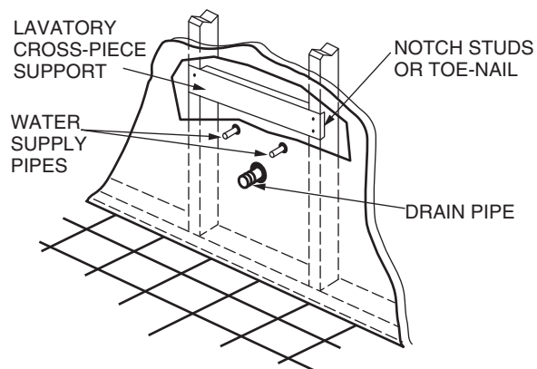
INSTALLING CROSS-PIECE
