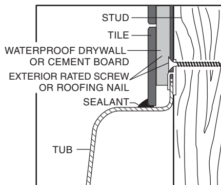
WOOD STUDS
