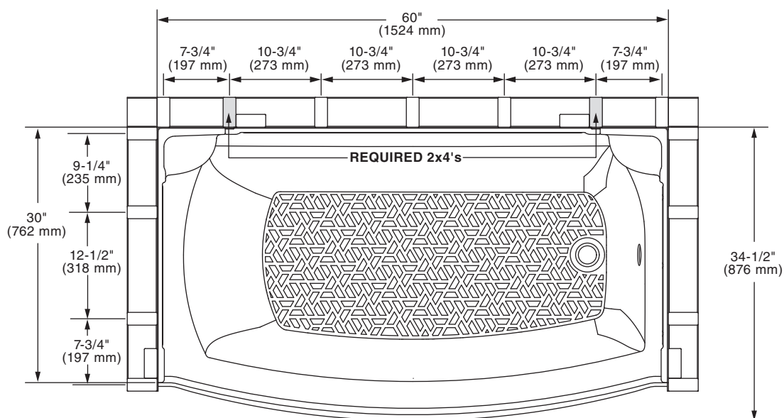
Alcove Stud Installation When Installing Ovation Shower Wall System
