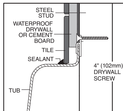
SUGGESTED BATH INSTALLATION METHOD
