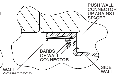
FIG. C CUTAWAY VIEW LOOKING DOWN FROM TOP
