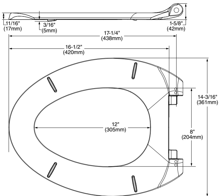
5503A65BH Elongated Toilet Seat
