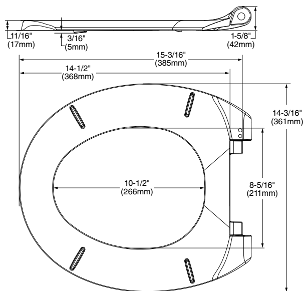
5503B65BH Round Front Toilet Seat
