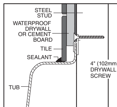
SUGGESTED BATH INSTALLATION METHOD
