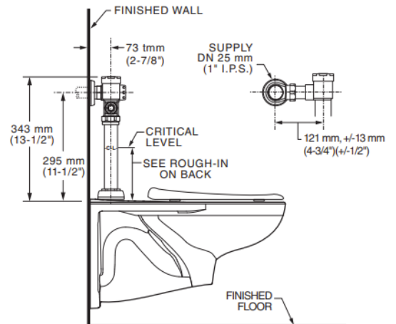
TYPICAL WATER CLOSET INSTALLATION: AFWALL™ TOILET SHOWN
